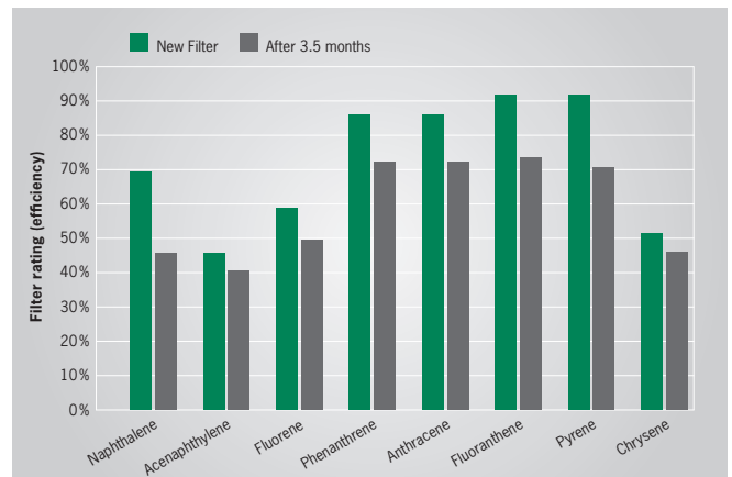
Test conducted in winter (outdoor air, ordinary ventilation plants in Stockholm).
