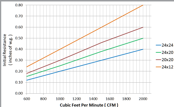
Initial resistance versus airflow, recommended velocity is 400 feet per minute or less to obtain published adsorbent efficiency.
